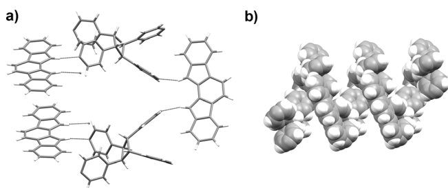
Figure 5. X-ray structure of (\text{IC})(4,4'\text{-tpcb}) : a) N–H···N forces between 4,4'-tpcb and IC, and b) space-filling model of the 1D structure.
